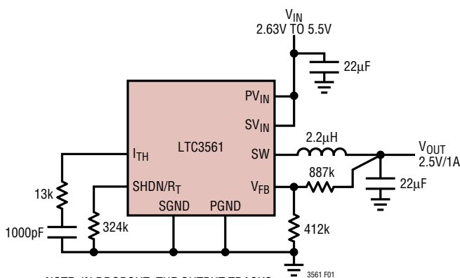
Step-Down 2.5V/1A Regulator
