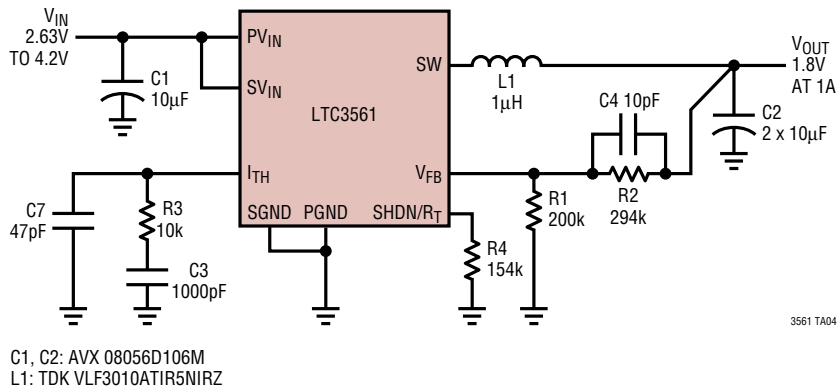
1mm Height, 2MHz, Li-Ion to 1.8V Converter
